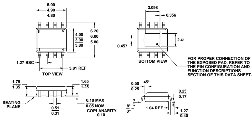
Figure 82. 8-Lead Standard Small Outline Package, with Exposed Pad [SOIC_N_EP]
