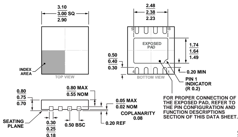
Figure 81. 8-Lead Lead Frame Chip Scale Package [LFCS_P_WD]
