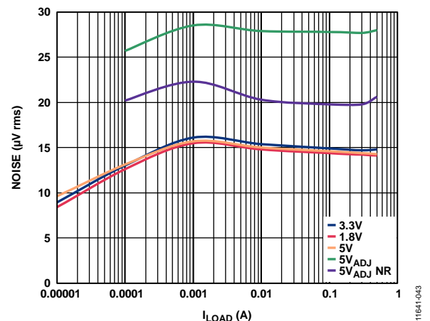
Figure 49. Output Noise vs. Load Current and Output Voltage, C_{OUT} = 1\text{ }\mu\text{F}
