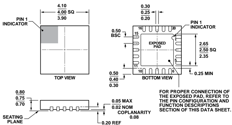
COMPLIANT TO JEDEC STANDARDS MO-220-WGGD. Figure 44. 20-Lead Lead Frame Chip Scale Package [LFCSP_WQ] 4 mm × 4 mm Body, Very Thin Quad (CP-20-10) Dimensions shown in millimeters
