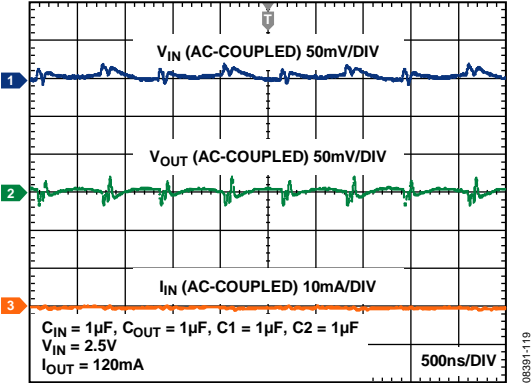
Figure 23. Typical Operating Waveforms, G = 2\times
