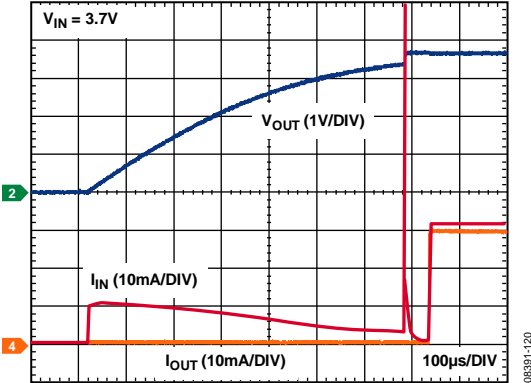
Figure 24. Typical Start-Up Waveform
