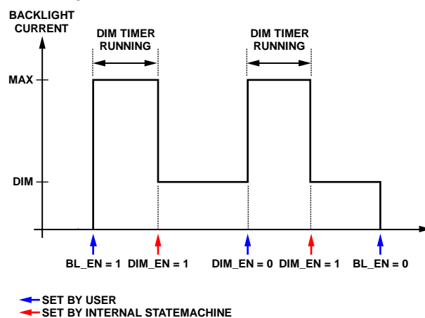
Figure 33. Dim Timer
