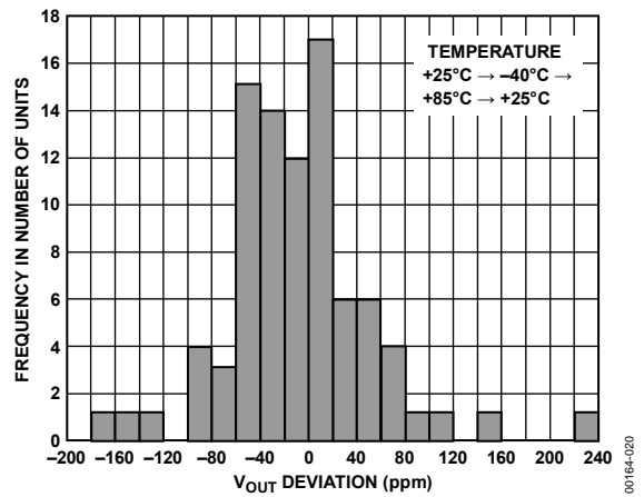
Figure 20. Typical Hysteresis for the ADR29x Product
