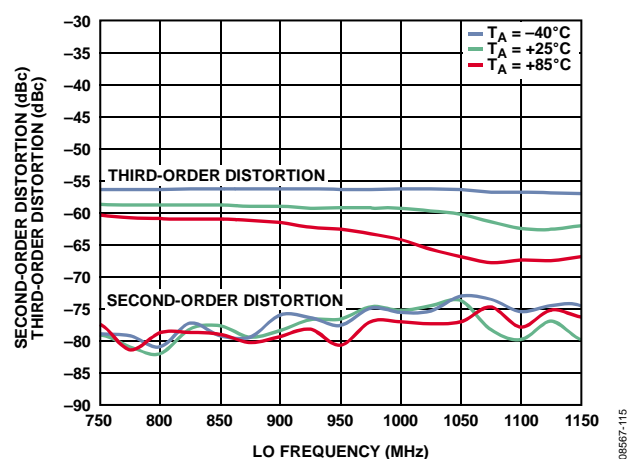
Figure 15. Second- and Third-Order Distortion vs. LO Frequency ( f_{LO} ) and Temperature
