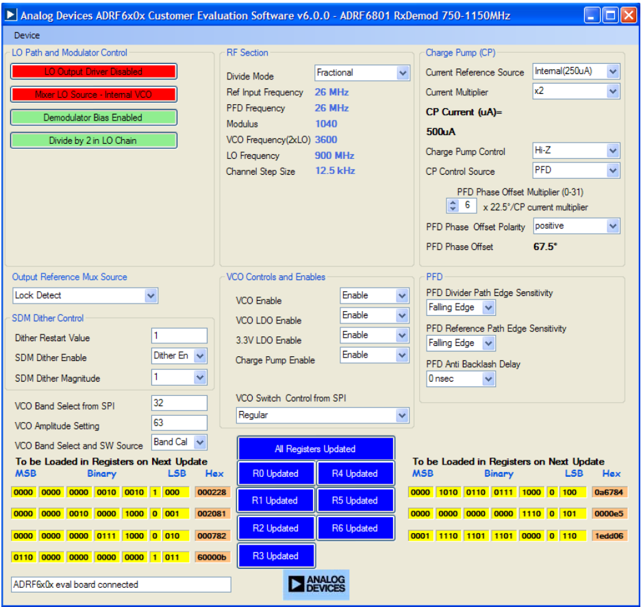
Figure 46. Evaluation Board Software Main Window
