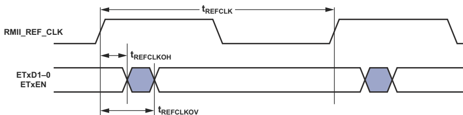
Figure 33. 10/100 Ethernet MAC Controller Timing: RII Transmit Signal
