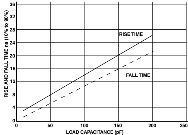
Figure 62. Typical Output Delay or Hold for Driver F at V_{DDEXT} \text{ Max}
