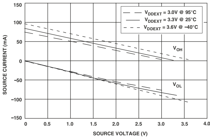
Figure 43. Drive Current D (High V_{DDEXT} )
