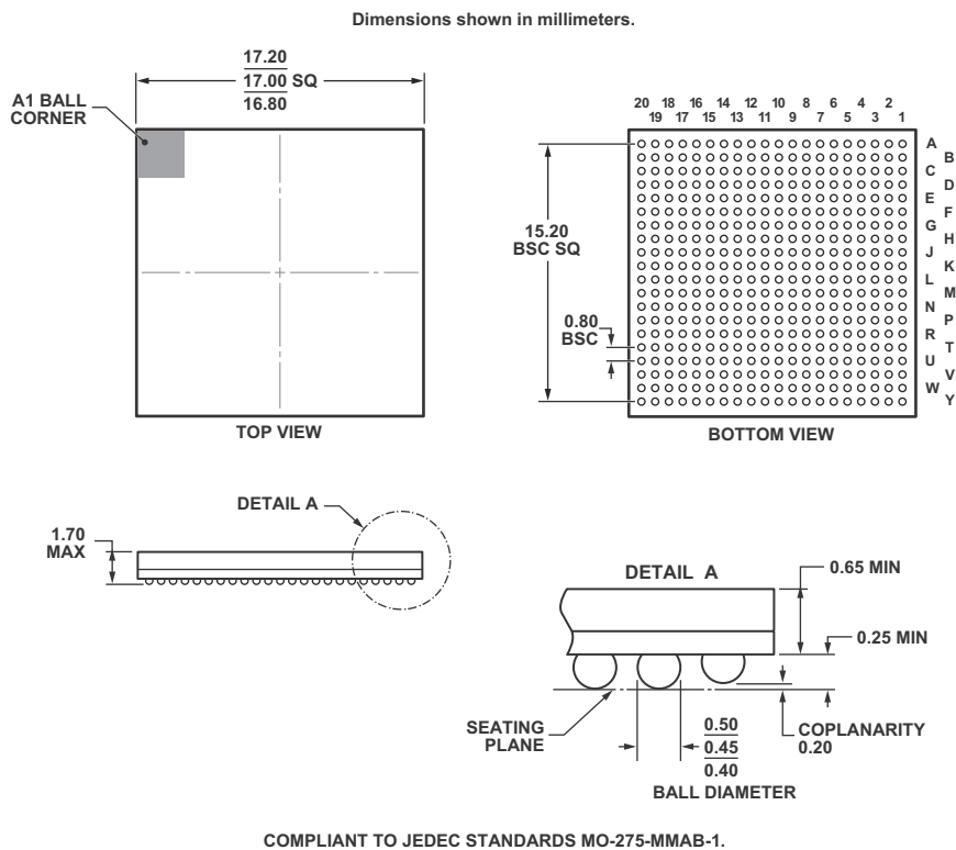
Figure 88. 400-Ball, 17 mm × 17 mm CSP_BGA (Chip Scale Package Ball Grid Array) (BC-400-1)
