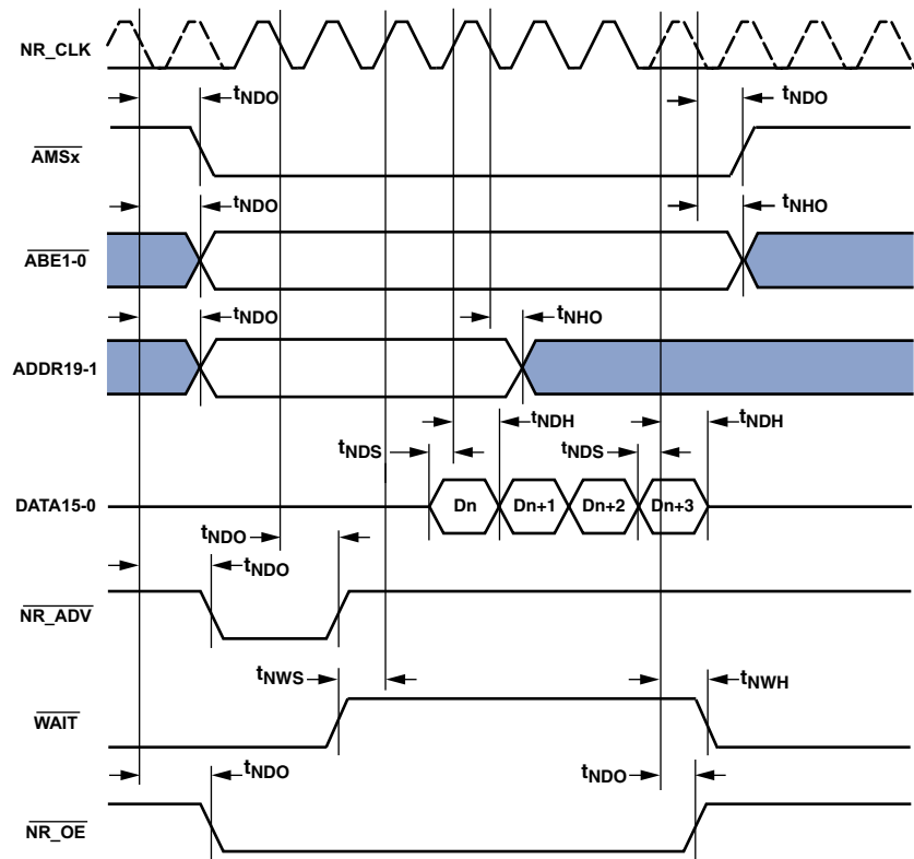
Figure 28. Synchronous Burst AC Interface Timing
