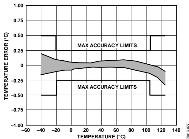
Figure 4. Temperature Accuracy at 3 V
