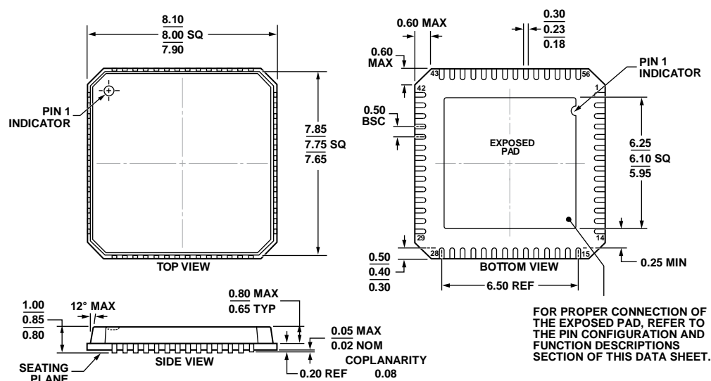
Figure 61. 56-Lead Lead Frame Chip Scale Package [LFCSQ_VQ] 8 x 8 mm Body, Very Thin Quad (CP-56-1)
