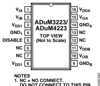
Figure 4. Pin Configuration
