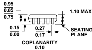
Figure 21. 10-Lead Mini Small Outline Package [MSOP] (RM-10) Dimensions shown in millimeters
