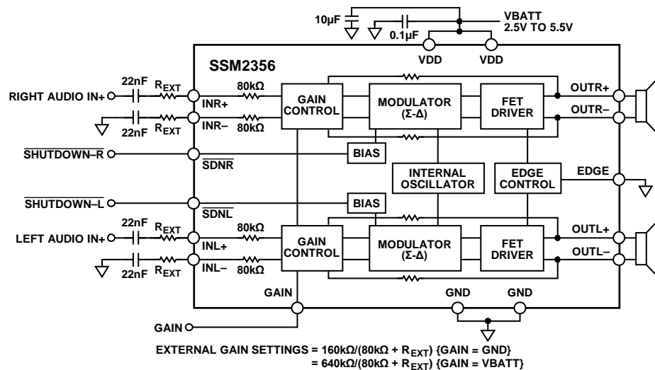
Figure 35. Stereo Single-Ended Input Configuration (When GAIN = VBATT use no larger than 10 kΩ R_{\text{EXT}} )
