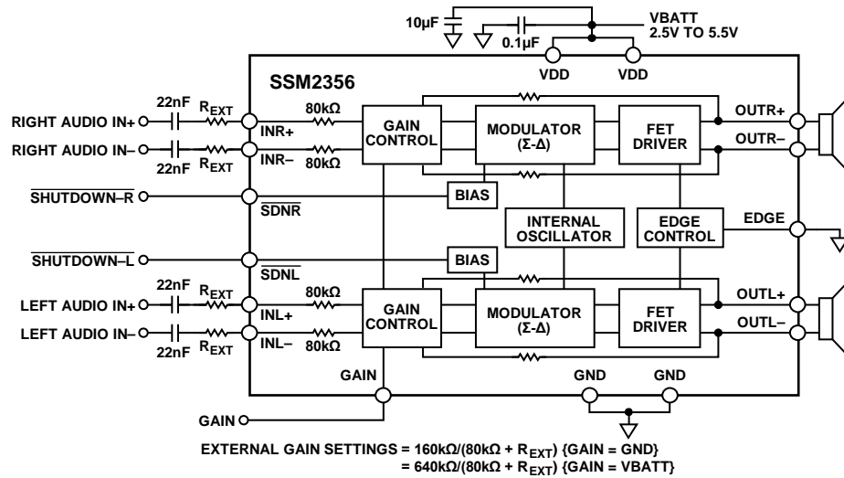
Figure 34. Stereo Differential Input Configuration (When GAIN = VBATT use no larger than 10 kΩ R_{\text{EXT}} )
