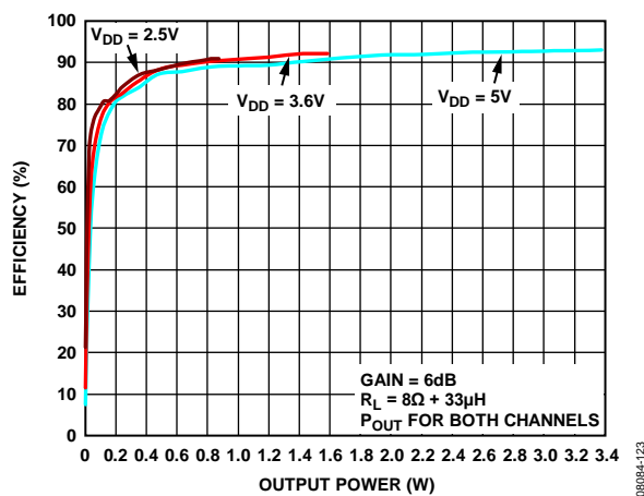
Figure 25. Efficiency vs. Output Power into 8\ \Omega
