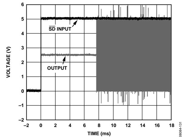
Figure 32. Turn-On Response
