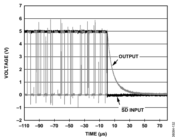
Figure 33. Turn-Off Response
