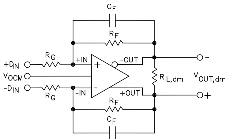
FIGURE 2. Circuit definitions.
