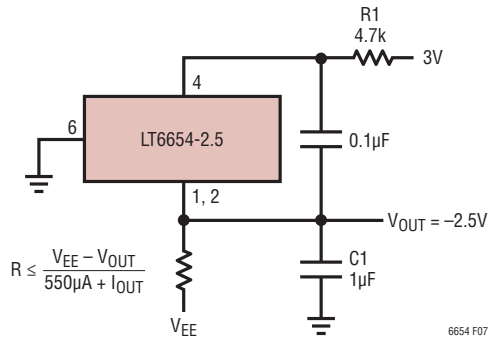
Figure 7. Using the LT6654-2.5 to Build a -2.5\text{V} Reference
