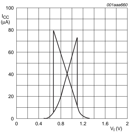
Fig 11. Typical 74LV14 transfer characteristics
