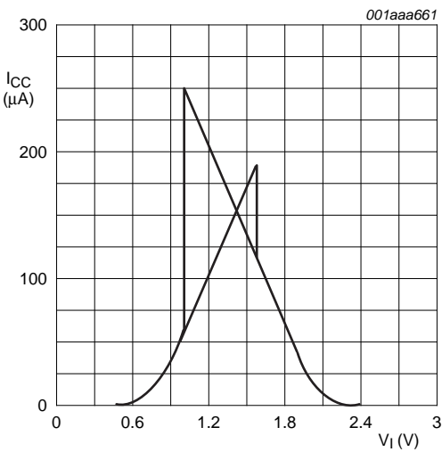
Fig 12. Typical 74LV14 transfer characteristics
