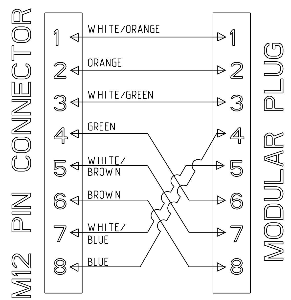
WIRING DIAGRAM SCALE 1:2
