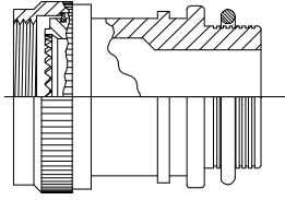
STRAIGHT ADAPTER
