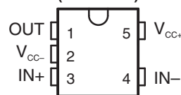
TL971...DBV PACKAGE (TOP VIEW)
