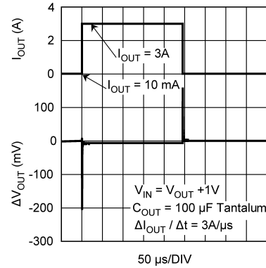
Load Transient Response, C_{OUT} = 100\ \mu\text{F Tantalum}
