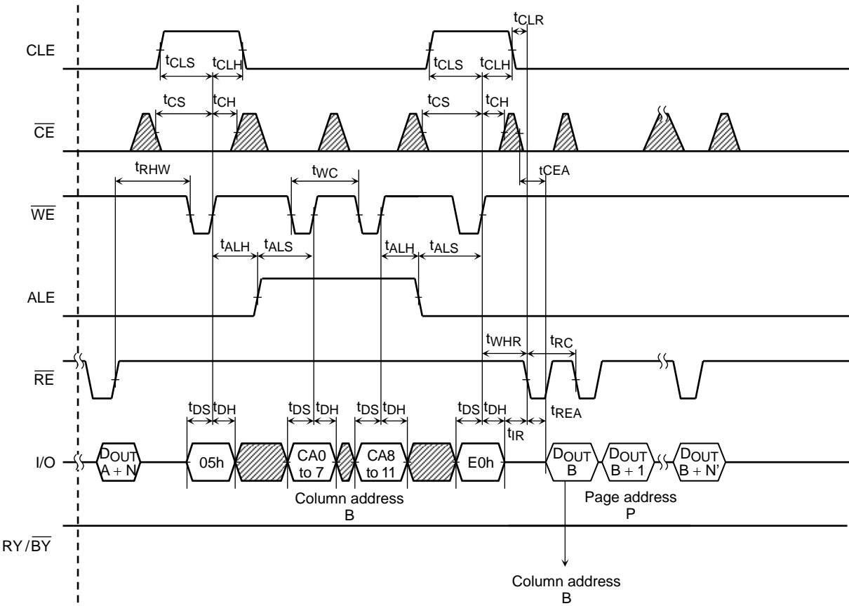
Column Address Change in Read Cycle Timing Diagram (2/2)
