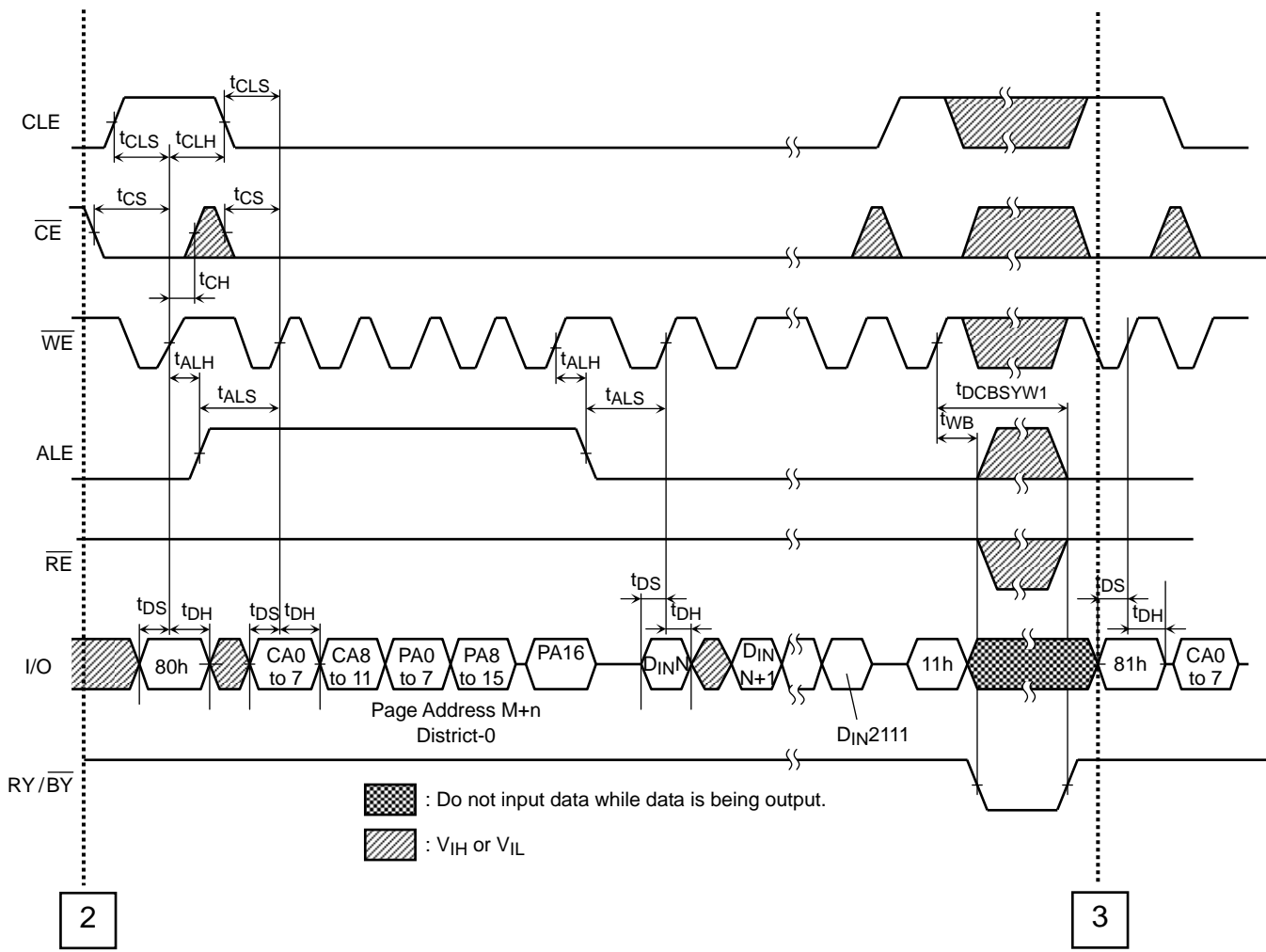
Multi-Page Program Operation with Data Cache Timing Diagram (3/4)
