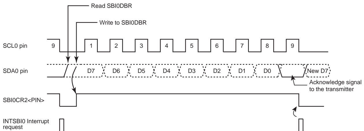
Figure 18-19 Example when SBI0CR1&lt;BC&gt;="000" and SBI0CR1&lt;ACK&gt;="1"
