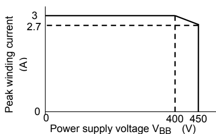
Figure 1 SOA at T_j = 135^\circ\text{C}
