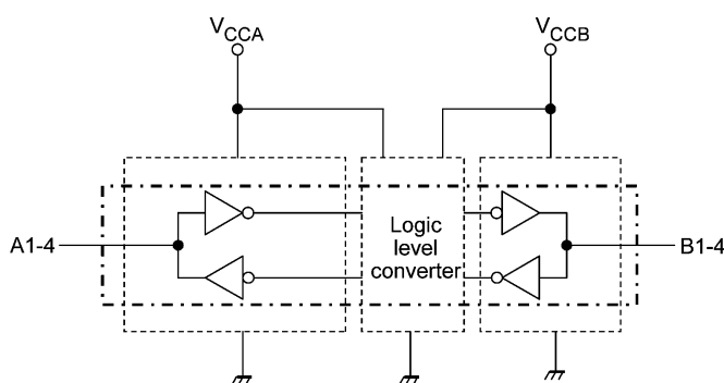
Fig. 6.1 Block Diagram
