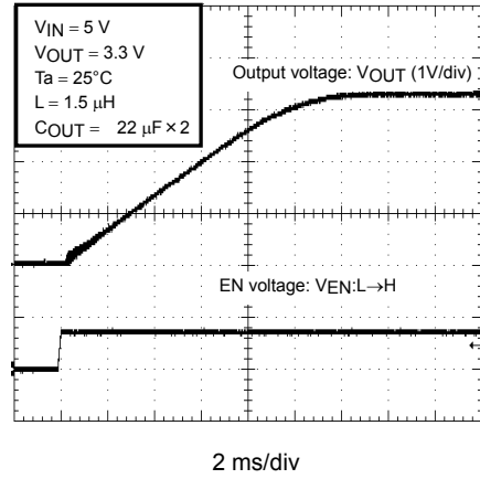
Startup Characteristics ( C_{SS} = 0.1\mu F )
