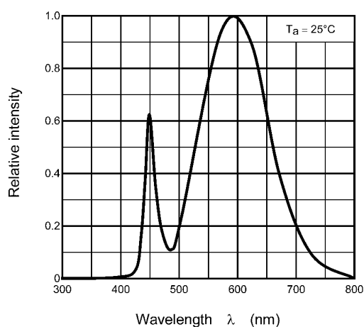
Fig. 8.4 Wavelength characteristic
