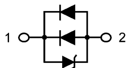
Fig. 13.1 Internal Circuit
