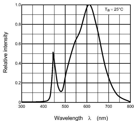
Fig. 8.4 Wavelength characteristic
