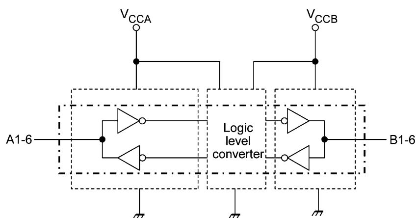
Fig. 6.1 Block Diagram
