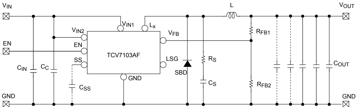
Figure 1 TCV7103AF Typical Application Circuit Examples
