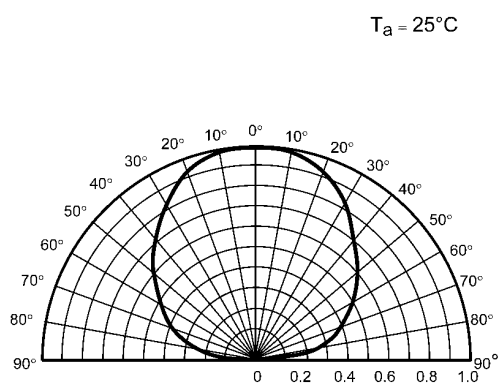
Fig. 8.5 Radiation Pattern
