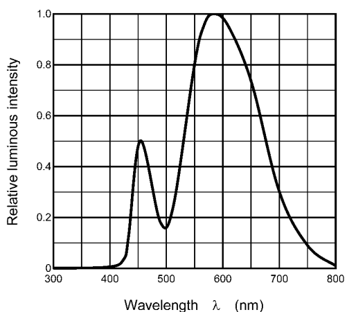
Fig. 8.6 Wavelength Characteristic
