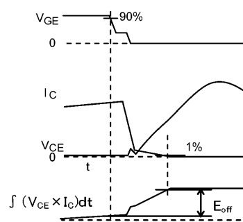
Fig. 6.2.4 Timing Chart of Switching Loss
