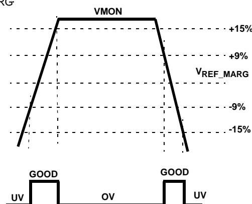
FIGURE 3. UNDERVOLTAGE-OVERVOLTAGE WINDOW
