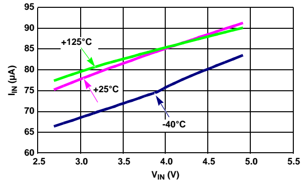
FIGURE 3. I_{IN} vs V_{IN} OVER TEMPERATURE
