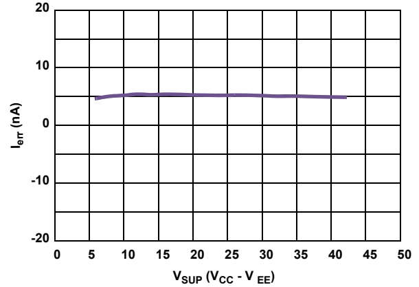
FIGURE 6. I_{ERR} vs SUPPLY VOLTAGE ( V_{CC} - V_{EE} )
