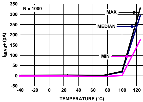
FIGURE 27. I_{BIAS+} vs TEMPERATURE, V_+ , V_- = \pm 1.2V
