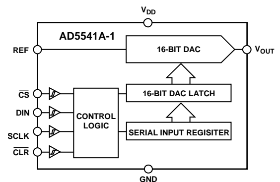
Figure 2. AD5541A-1
