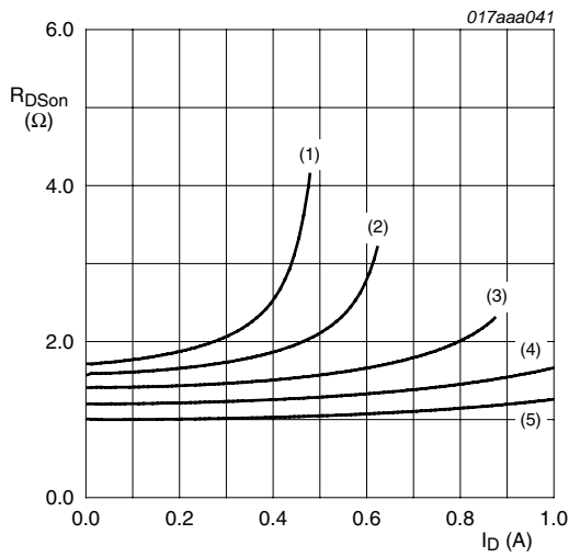
Fig 8. Drain-source on-state resistance as a function of drain current; typical values Tamb = 25 °C (1) VGS = 3.25 V (2) VGS = 3.5 V (3) VGS = 4 V (4) VGS = 5 V (5) VGS = 10 V
