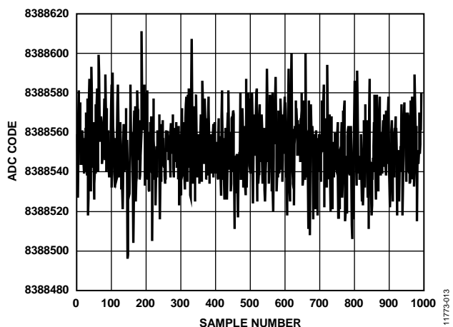
Figure 13. Noise (Output Data Rate = 31.25 kSPS, Analog Input Buffers Enabled)
