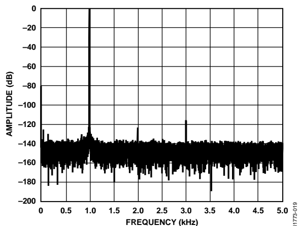
Figure 19. ADC Output FFT; 1 kHz Input Tone, -0.5 dBFS Input FFT (Output Data Rate = 10 kSPS, External Reference, External Clock, Buffers Enabled)
