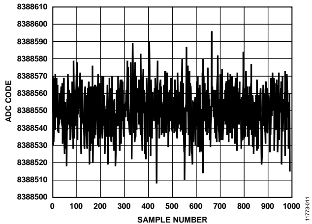
Figure 11. Noise (Output Data Rate = 10 kSPS, Analog Input Buffers Enabled)
