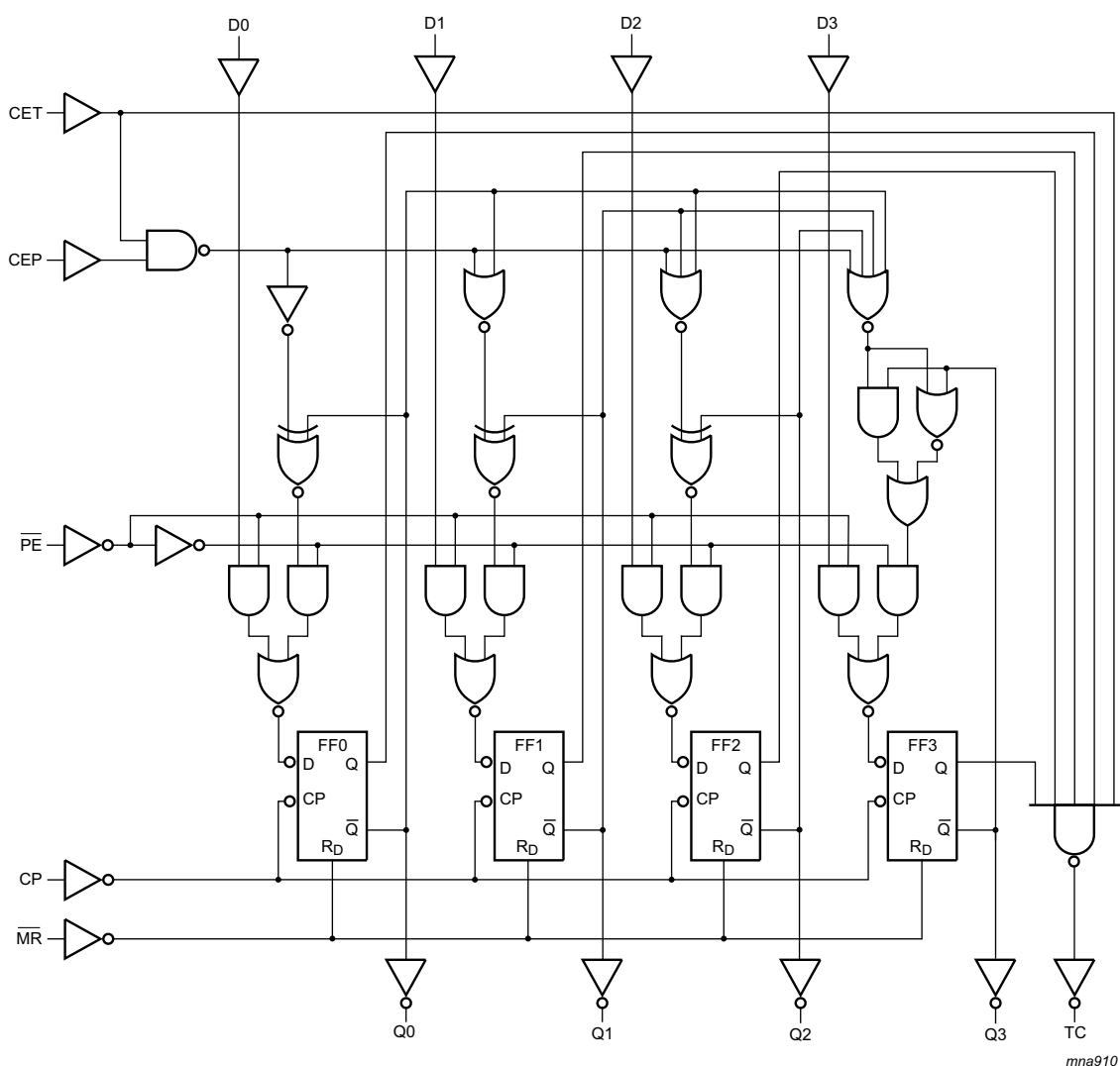
Fig 8. Logic diagram
