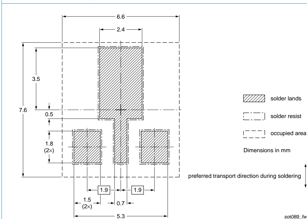
Fig 29. Wave soldering footprint SOT89 (SC-62/TO-243)
