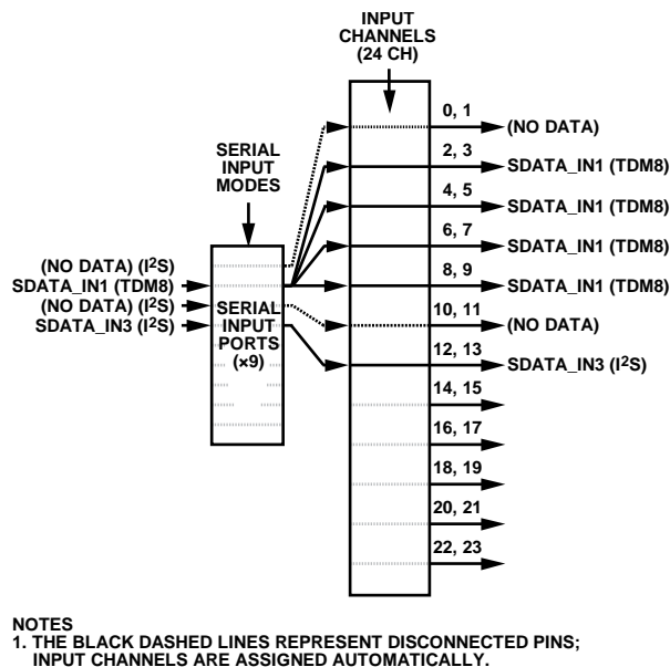
Figure 38. Automatic Input Channel Assignment Example with Skipped Pins
