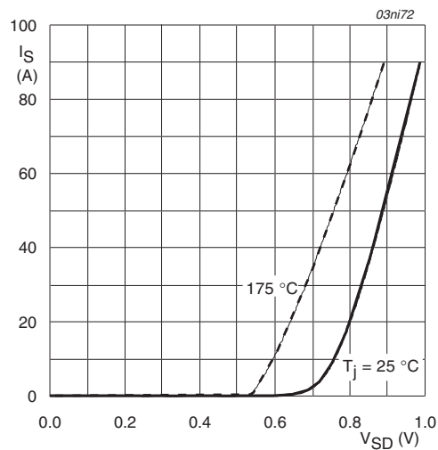
Fig 16. Reverse diode current as a function of reverse diode voltage; typical values
