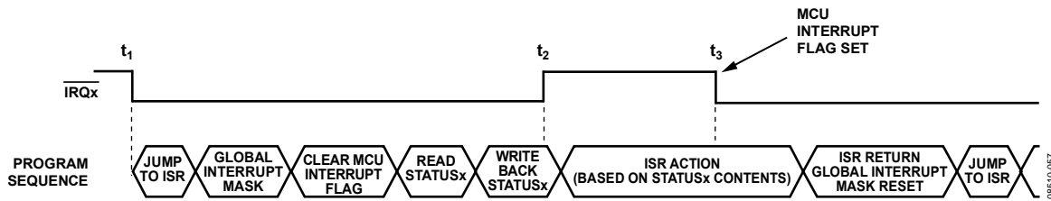
Figure 84. Interrupt Management
