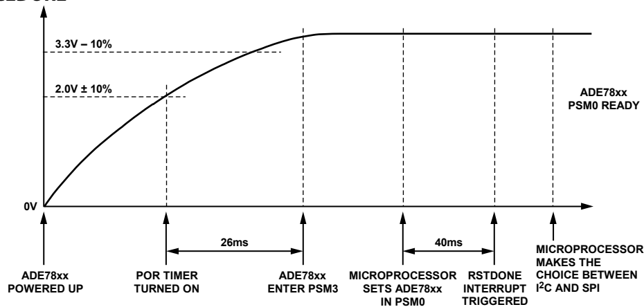
Figure 26. Power-Up Procedure
