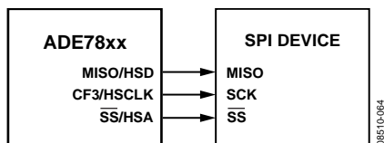
Figure 91. Connecting the ADE78xx HSDC with an SPI
