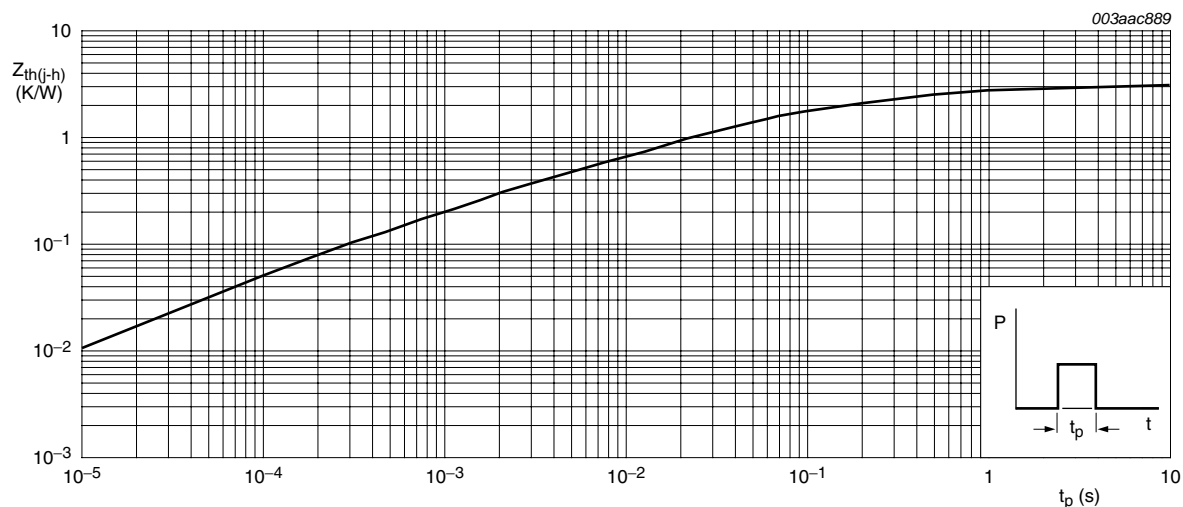
Fig 3. Transient thermal impedance from junction to heatsink as a function of pulse width
