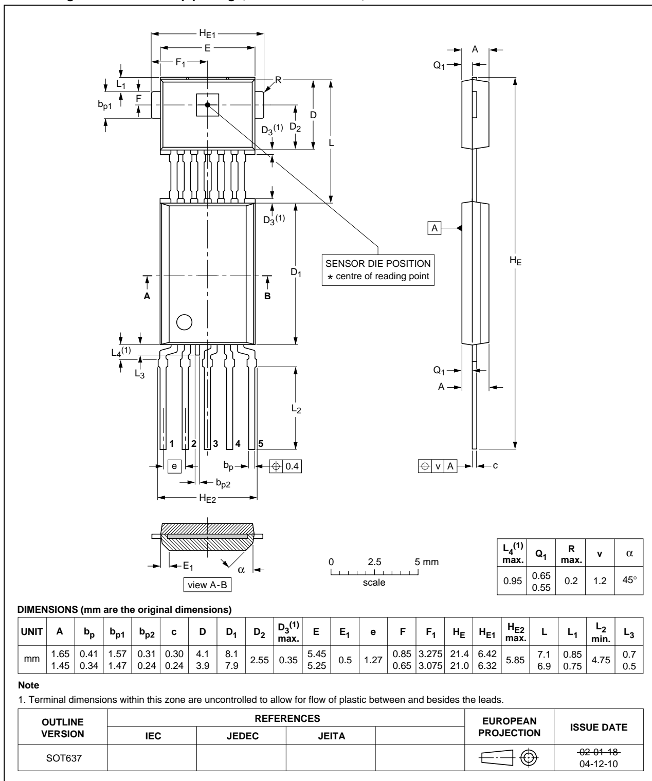
Fig 13. Package outline SOT637
