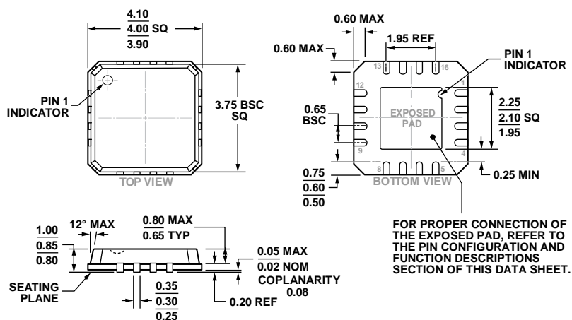
Figure 49. 16-Lead Lead Frame Chip Scale Package [LFCSP_VQ] 4 mm x 4 mm Body, Very Thin Quad (CP-16-4) Dimensions shown in millimeters
