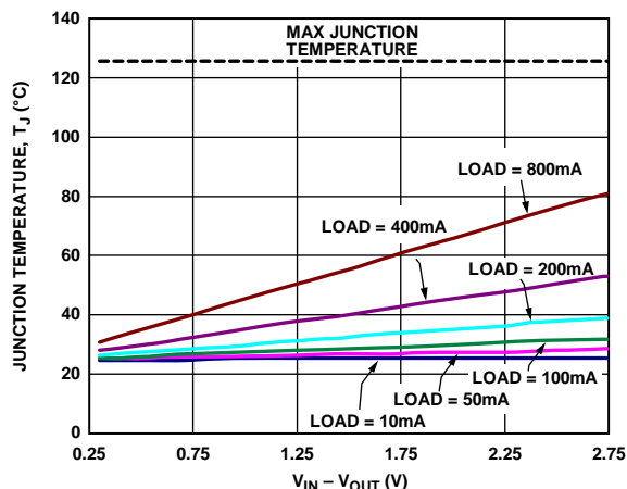
Figure 44. 1000 mm² of PCB Copper, T_B = 25^\circ\text{C} , LFCSP
