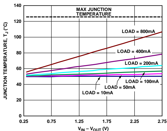
Figure 45. 1000 mm² of PCB Copper, T_B = 50^\circ\text{C} , LFCSP
