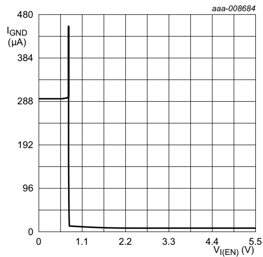
Fig 10. Ground current versus input voltage on pin \overline{EN}
