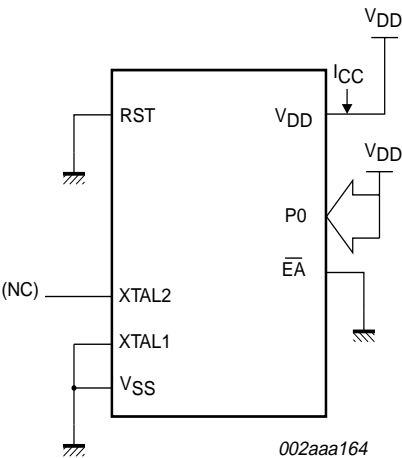
Fig 16. I_{CC} test condition, power-down mode (all other pins are disconnected, V_{DD} = 2.0 \text{ V to } 5.5 \text{ V} ).
