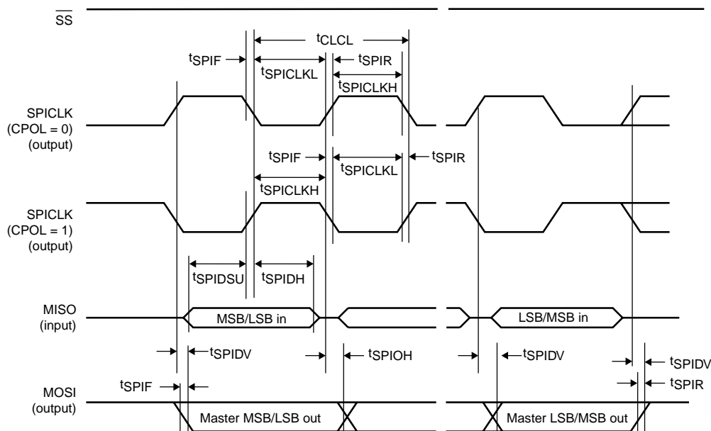
Fig 9. SPI master timing (CPHA = 1).
