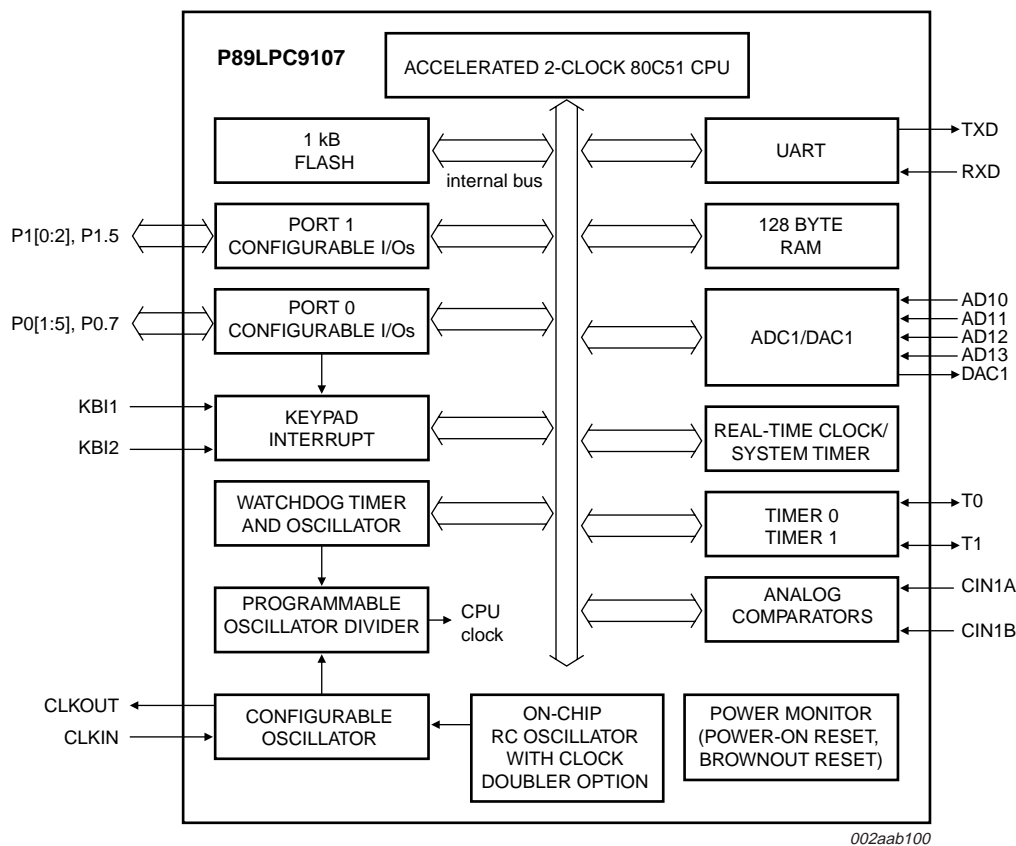
Fig 3. Block diagram of P89LPC9107
