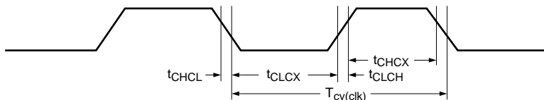
Fig 34. External clock drive waveform (with an amplitude of at least V_{i(RMS)} = 200 mV)
